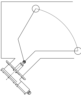
Radial movement for angle design (Fig.5)
