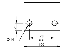
View "B" (Bracket available for types 7-8)
