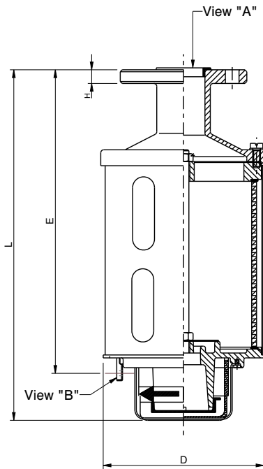
View "B" (Bracket available for types 7-8)
